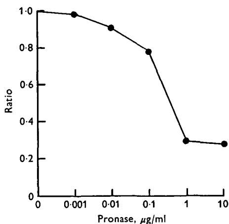
Fig. 14. The effect of pronase on the sedimentation of HeLa nucleoids.
