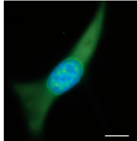
Fig. 2. Poly(A) + RNA in the nucleus and cytoplasm. Little poly(A) + RNA is found at the nuclear periphery in a mouse fibroblast (NIH 3T3). Poly(A) + RNA was detected by in situ hybridization using biotinylated poly(dT) 54 and streptavidin conjugated with Alexa594 (pseudo-coloured green); DNA was counterstained with DAPI (blue). Image kindly provided by Meg Byron, John McNeil and Jeanne Lawrence. Bar, 10 \mu m.
