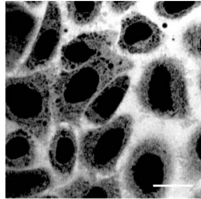
Fig. 3. The nuclei (but not cytoplasm) of permeabilized HeLa cells exclude a 40 kDa dextran conjugated with fluorescein isothiocyanate (FITC). HeLa cells were permeabilized in saponin in a 'physiological' buffer, washed in the same buffer, incubated (15 minutes, 27.5°C) in the precursors required for translation (as for Fig. 2 of Iborra et al., 2001), a 40 kDa dextran-FITC added, and cells imaged on a confocal microscope. FITC fluorescence is illustrated. Bar, 10 µm.
