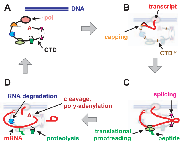
Fig. 4. A model for transcript production (Iborra et al., 2004). (A) The CTD has the potential to associate with sites involved in capping, transcript degradation, translational proofreading (involving the translational and NMD machineries), proteolysis, splicing and polyadenylation. It remains unclear whether all bind to the CTD simultaneously, or whether they attach and detach as needed. [Wetterberg et al. (Wetterberg et al., 2001) have analysed the association of the splicing machinery during the synthesis of an exceptionally long mRNA.] (B) Transcription began as the template bound to the polymerizing complex and was reeled in as the transcript was extruded; the CTD is now hyper-phosphorylated (CTD P ), and a cap has been added. (C) The transcript continues to be extruded through a splicing site as the ribosome/NMD machinery begins proofreading the now-spliced message (and so does not read introns, which might contain many termination codons). (D) Once introns are removed (lariat), the transcript is cleaved and poly-adenylated, and is ready to leave for the cytoplasm. If errors are detected, the faulty transcript and peptide produced during proofreading are degraded by nucleases and proteasomes.
