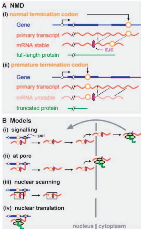
Fig. 1. Nonsense-mediated decay. (A) The phenomenon. The gene (with promoter, parts of the first and penultimate exons, and last exon), primary transcript, spliced mRNA (with an exon junction complex – EJC – deposited 5' of the exon-exon junction) and protein are shown. UPF proteins associate with the EJC (not shown). (i) Transcription of a gene with a termination codon in the correct place leads to a spliced and stable mRNA, and a full-length protein. (ii) Moving the termination codon 5' to what will become an exon-exon junction leads to an unstable mRNA and a truncated protein. (B) Models for NMD. In each case, an mRNA encoding a PTC is made at the transcription site by a polymerase (pol). The mRNA with its EJC then passes through the nucleoplasm to dock at the membrane, before exiting through the pore to the cytoplasm. The mRNA is destroyed once the NMD machinery detects the PTC. (i) A cytoplasmic ribosome detects the PTC, and transmits a signal to the nucleus that leads to degradation of homologous transcripts containing the PTC. (ii) NMD occurs as the transcript bearing the PTC emerges into the cytoplasm. (iii) Some unknown nuclear mechanism (black box) recognizes the PTC and destroys the mRNA. (iv) A ribosome detects the PTC in the nascent transcript at the transcription site.
