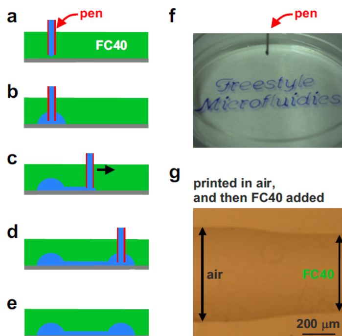
Supplementary Figure 3. Creating simple circuits under FC40.
