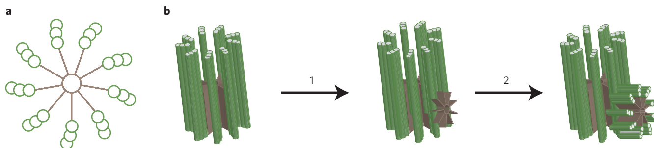
Figure 1 | A schematic view of centrioles and the early stages of centriole duplication. (a) An end-on view of a centriole showing the nine-fold symmetry of the central hub and spokes of the cartwheel structure (gray) and the surrounding 'blades' of triplet microtubules (green). In some species and cell types, only doublet or singlet microtubules surround the cartwheel: nine-fold symmetry is conserved in virtually all centrioles. (b) During S phase, the two centrioles in a cell each duplicate (for simplicity, a single centriole is shown here). The precise structural details of centriole duplication are poorly understood, but the formation of a new cartwheel structure at right angles to the existing 'mother' centriole is thought to be an important early step (1), and this cartwheel is then rapidly surrounded by new microtubules (2). During S and G2 phases, the new centrioles elongate until they are approximately the same size as the original mother centriole (not shown), and in most species the cartwheel structure is ultimately restricted to the proximal end of the centrioles (as illustrated for the mother centriole shown here).
