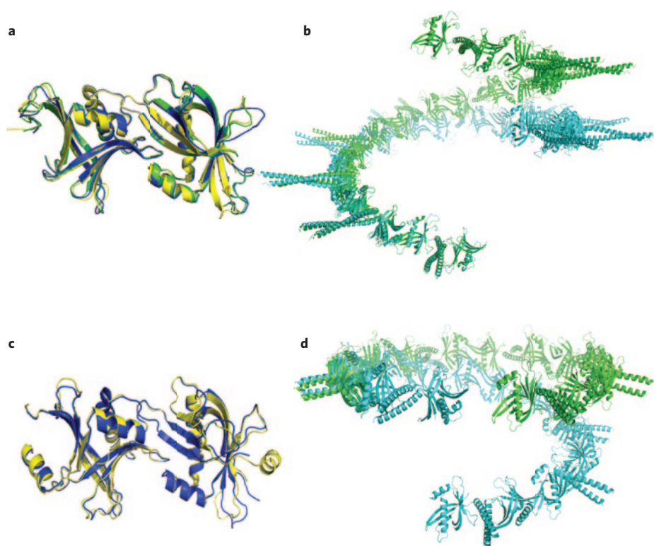
Figure 3 | An illustration of the distinct SAS-6 oligomer models that can be derived from slightly different dimer orientations observed in the SAS-6 crystal structures. All models are further described in Table 1 . (a) Three slightly different head-group dimers were present in the CrSAS-6 N terminus (PDB code 3Q0Y) structure. Here, dimers CD (yellow) and EF (blue) are superimposed upon dimer AB (green). Average r.m.s. deviation between the dimers = 0.6 \pm 0.1 Å over 1,876 \pm 14 atoms. (b) Two models of CrSAS-6 dimer oligomers were assembled (in a clockwise manner) using the A→B orientation of the coiled-coil dimer shown in PDB entry 3Q0X and either the 3Q0Y C→D (green) or the 3Q0Y B→A (blue) orientation of the head group. Both models generate a left-handed helical structure with approximately ten dimers per helical turn, but each has a different helical pitch. (c) Similar overlays shown for the two head-group dimers (AC and BD) present in the DrSAS-6 N-terminus crystal (r.m.s. deviation = 0.8 Å over 1,975 atoms). (d) Two models of DrSAS-6 dimer oligomers were assembled (in a clockwise manner) using the 2Y3W A→B orientation of the coiled-coil dimer and either the 2Y3V A→C (green) or B→D (blue) orientation of the head group. The first model generates a nearly circular arrangement of dimers (eight dimers are shown), whereas the second model generates a left-handed helical structure with eight to nine dimers per helical turn.
