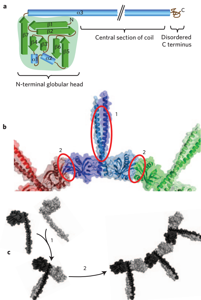
Figure 2 | The architecture and interactions of SAS-6. (a) Schematic representation of the overall topology of the SAS-6 family of proteins. (b) A schematic representation of the coiled-coil interaction (1) that occurs via the knob-and-holes packing of the coiled-coil tails and the head-group interaction (2) that is mediated by the hydrophobic plug residue. (c) A model of SAS-6 oligomerization: CrSAS-6 monomers initially dimerize via the coiled-coil interaction, and the resulting dimers can then associate via the head-group interaction to form circular oligomers.
