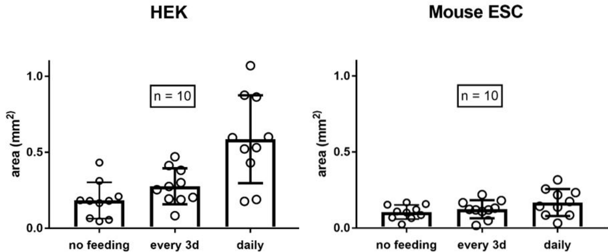
Figure S3. Size of colonies. Cells were cloned and fed as described in Figure S2 , and areas occupied by clones scored in the images collected after 8 days. Areas occupied by the clones are as expected, and the different feeding regimes have marginal effects on colony size. This indicates that the 400 nL media in a chamber is nevertheless sufficient to support early clonal growth.
