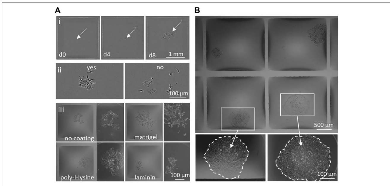
Figure 5. Cloning in chambers (1.9 × 1.9 mm) with fluid walls. (A) HEK cells. (i) Images of a whole chamber containing a single cell that develops into a colony over 8 days. The single cell seen at d0 moves slightly to the right in d4, prior to forming the colony. (ii) An arbitrary threshold (i.e., ≥16 cells derived from one progenitor) is used to define a colony; only the colony on the left meets this criterion. (iii) Fluidic chambers can be created on substrates ± different coatings (each pair of images shows a view of the complete chamber on the left and zoom on the right). Coatings visibly affect the morphology of colonies, which ranges from compact (poly-L-lysine) to spread out (Matrigel). (B) Mouse ES cells grow as more compact colonies than HEK cells, imaged using a 4× objective. The upper image shows a view of four chambers, each containing an 8-day-old colony derived from a single cell; zooms are shown below (dotted lines indicate colony limits). Edge effects are more pronounced here due to the addition of media for feeding, thereby increasing the GRIDs' contact angles (see Theory) resulting in the shaded regions around the edges. Single cells were identified prior to the addition of media.
